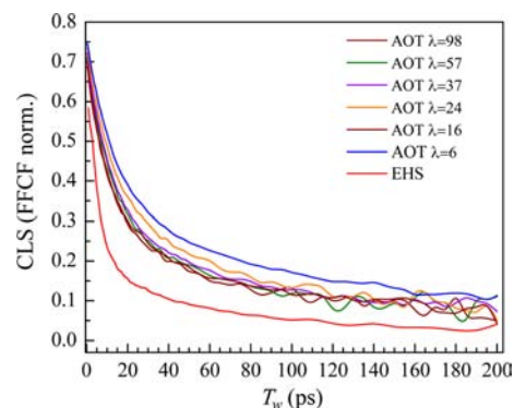
Figure 5. CLS curves for the CO stretching mode of W(\text{CO})_6 in AOT/water binary mixtures in the lamellar phase, \lambda = 98 to 16, in the BC phase, \lambda = 6 , and in the model liquid bis(2-ethylhexyl) succinate (EHS).
